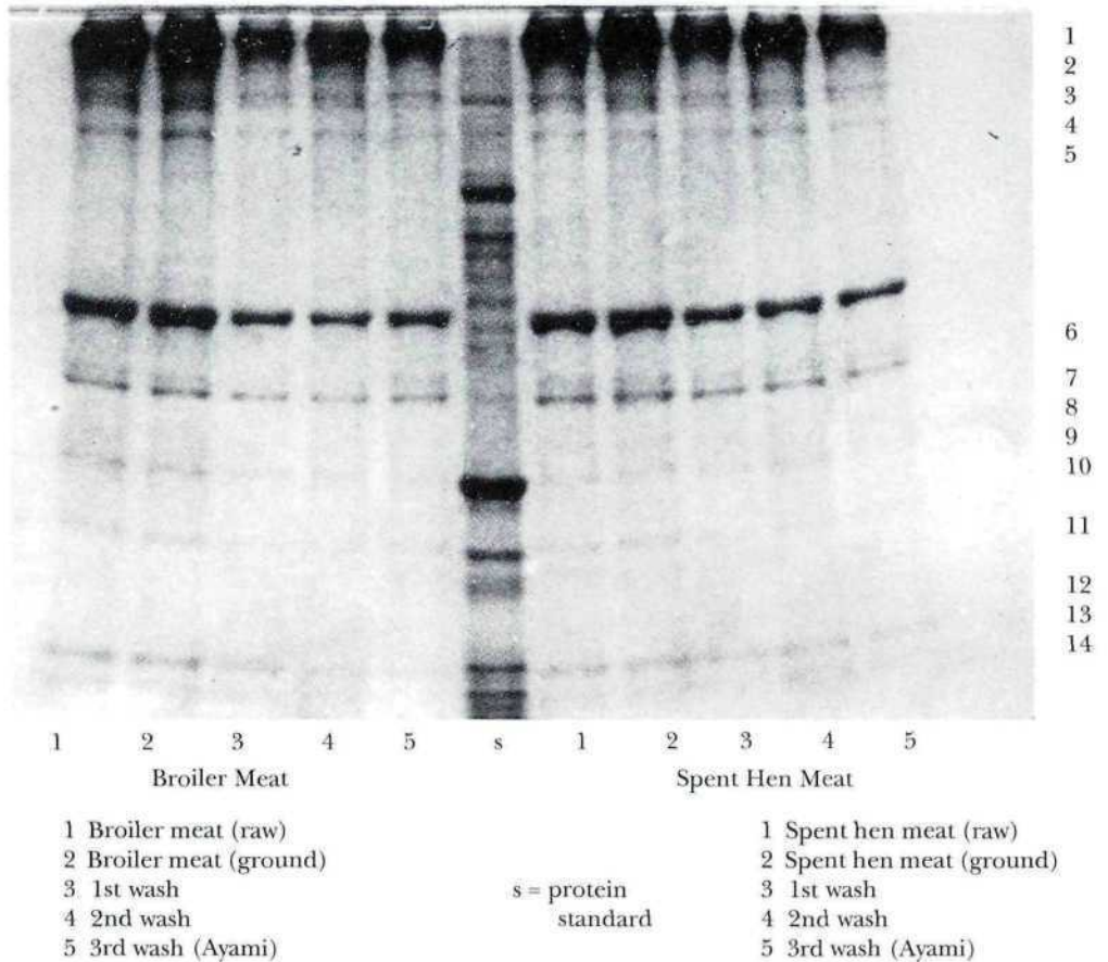
Fig. 3: Changes in myofibrillar proteins of broiler and spent hen meat due to various washing and processing procedures
