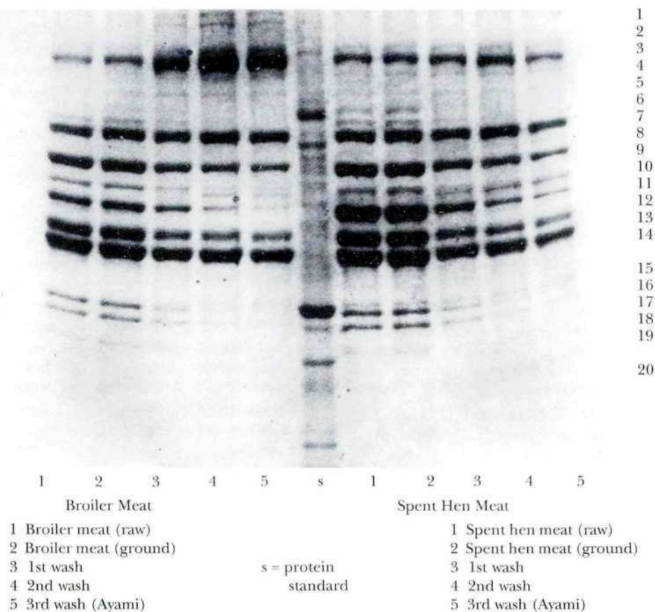
Fig. 2: Changes in sarcoplasmic proteins of broiler and spent hen meat due to various washing and processing procedures
